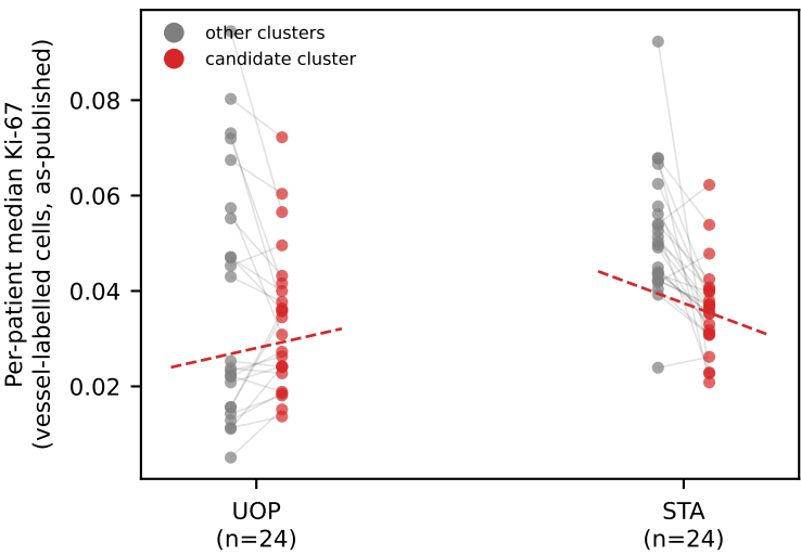
D Ki-67: candidate-cluster vessel cells vs other-cluster vessel cells (paired patients)
