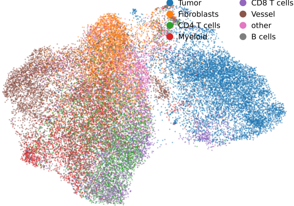
A2 Published cell labels (same cells)
