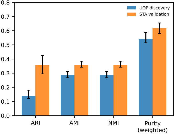
C External recovery of published labels (patient-level bootstrap 95% CI, B=500)
