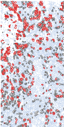
F2 Cell outlines red=candidate vessel; grey=other vessel; blue=others
