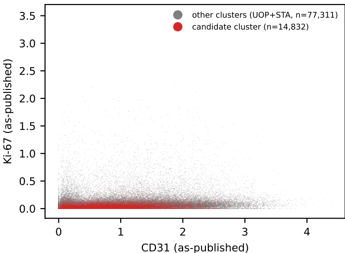
E Single-cell CD31-Ki-67 joint distribution (vessel-labelled cells; grey=other, red=candidate)
