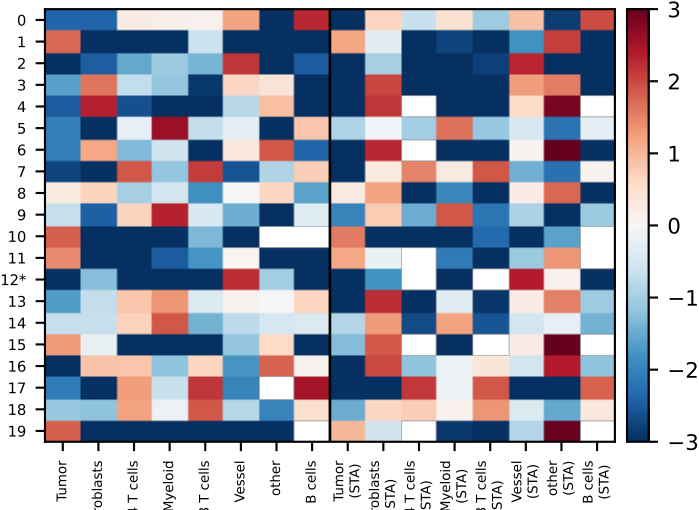
B Cluster × cell-type enrichment log2 obs/exp (*=candidate; left UOP, right STA)
