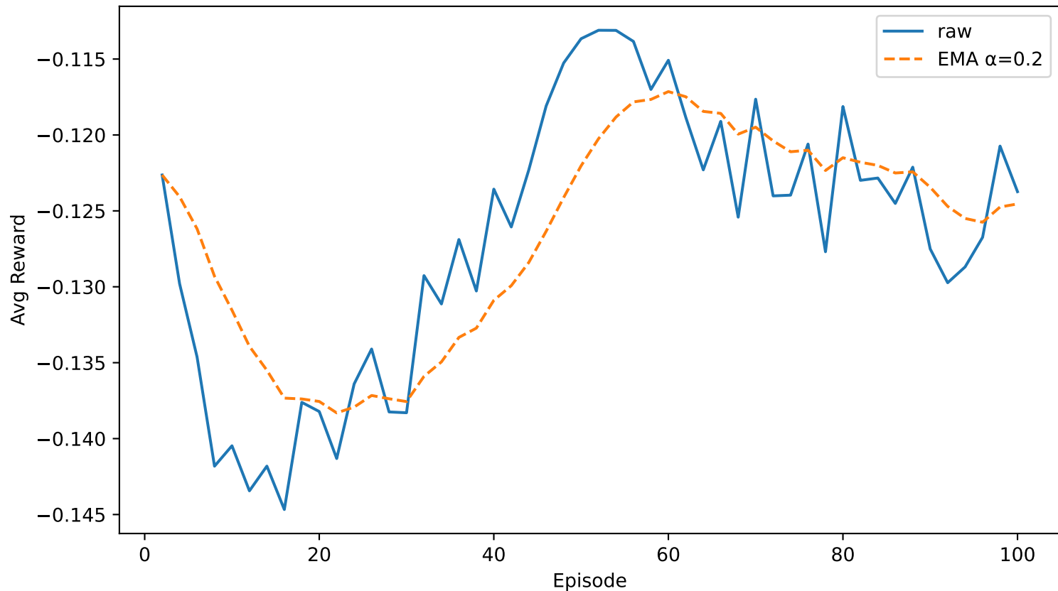
Low-Level Average Reward
