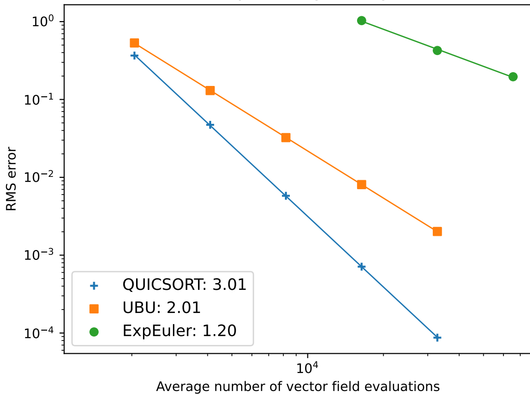
'Titanic' Bayesian Logistic Regression
