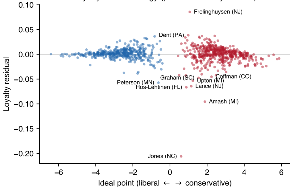
Loyalty is not ideology ( \rho with extremity = -0.04)
