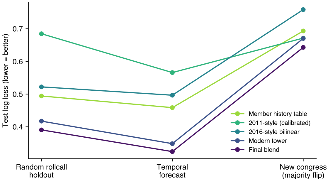
The same models under three forecasting regimes
