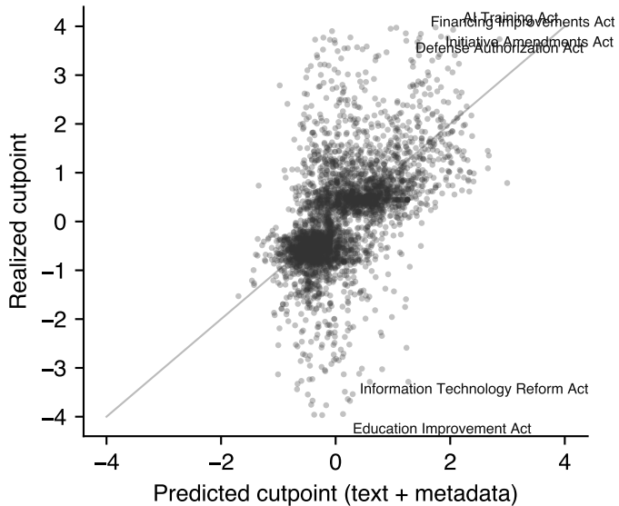
Held-out future rollcalls ( r = 0.55 )
