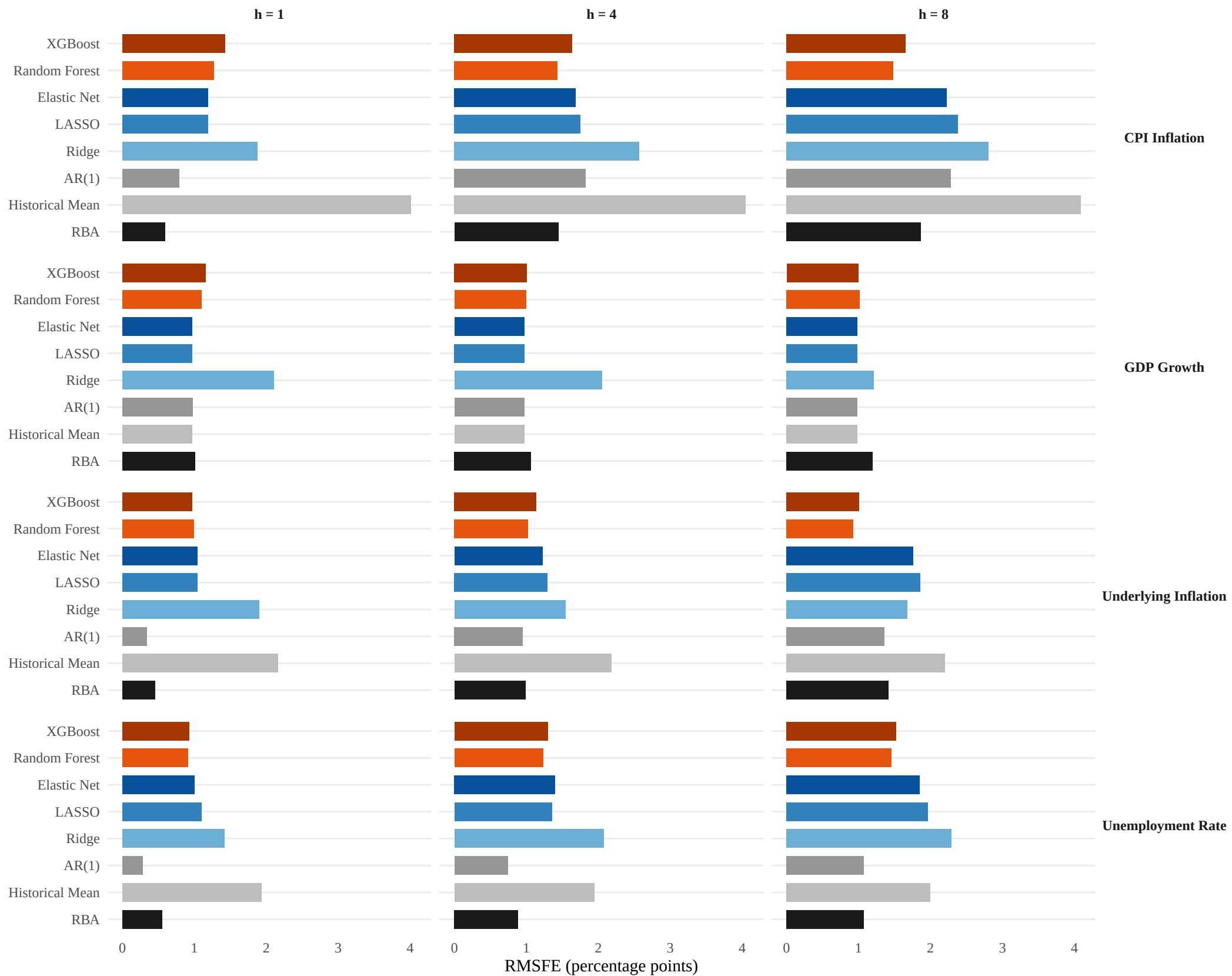
Root Mean Squared Forecast Error by Model and Horizon
