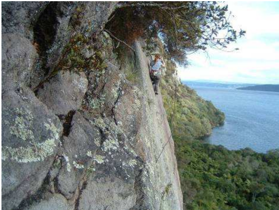
Kawakawa Bay
