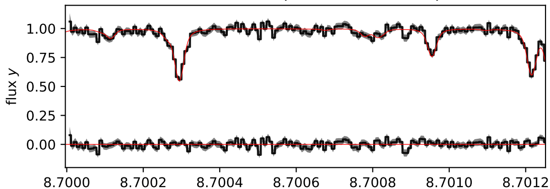
Frizzle combined spectrum (well-sampled)
