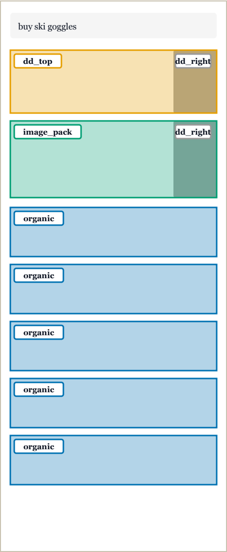
Labels via heading text → class → data-attrid chain. 13 element types incl. off-axis dd_right.
