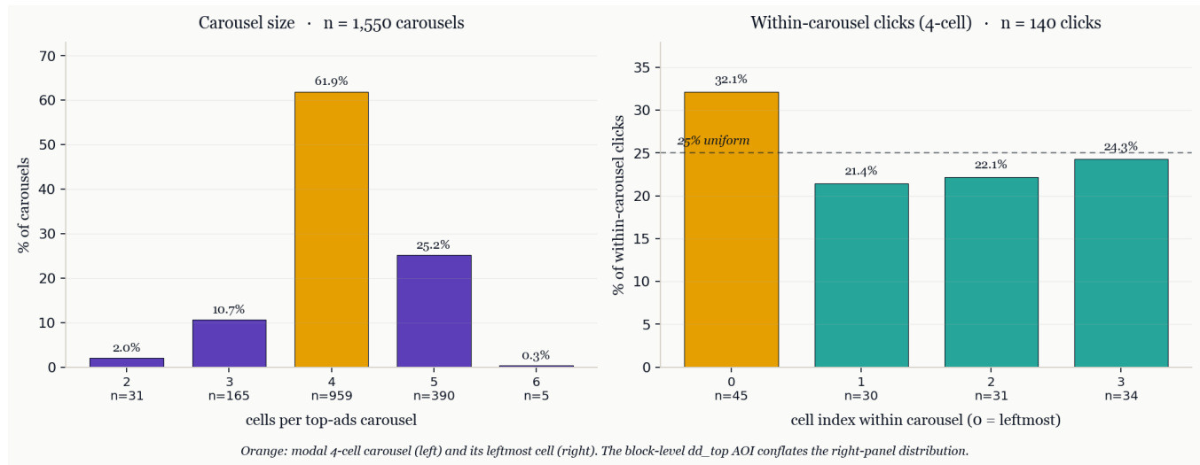
Figure 4: Anatomy of the top-ads cell split. Left: carousels hold 2 to 6 cards, modal 4 (61.9% of the 1,550 carousels the cell snapshot resolves). Right: of the 235 final clicks landing inside a carousel in the released export, the distribution on the modal four-cell layout ( n = 140 ) favours the leftmost cell (32.1% against a 25% uniform baseline) but spreads across all cells.
