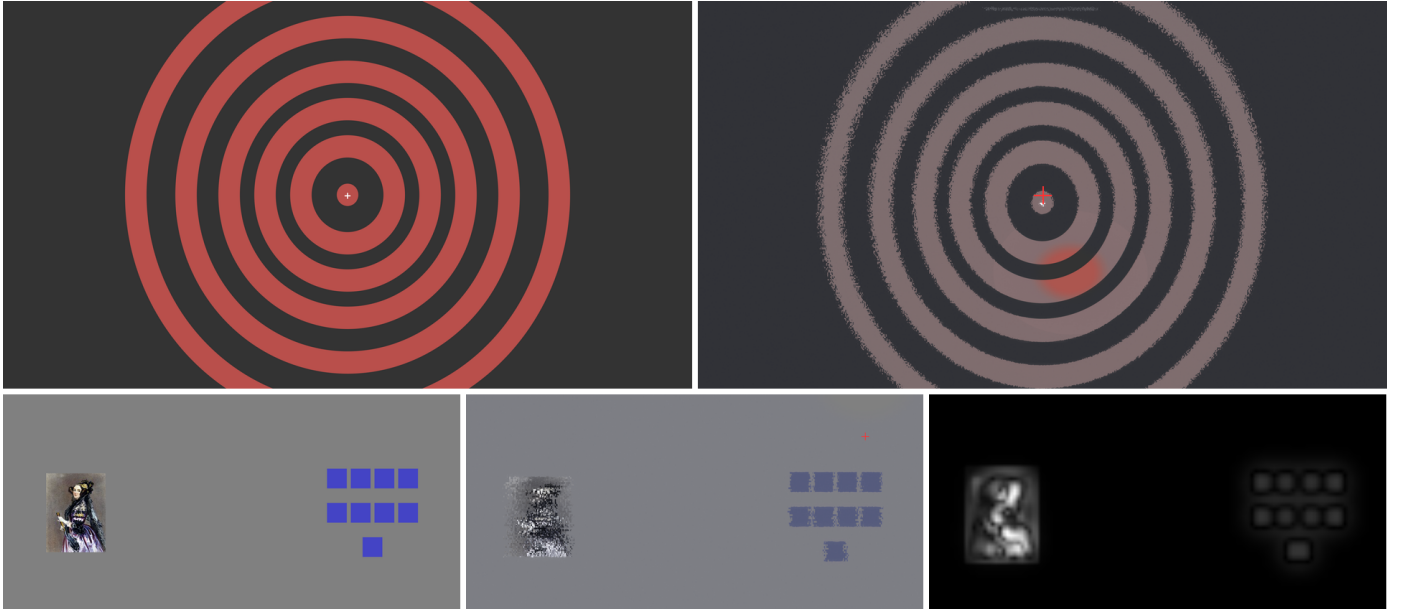
Figure 2: Pipeline output for two validation domains. Top: Chromatic decay, baseline (left) vs. filtered (right, fixation at red crosshair). Outer rings lose red-green chroma while blue-yellow structure persists, consistent with differential cone-opponent decay [Mullen and Kingdom, 2002]. Bottom: Saliency protection (cropped to face and control regions), three panels: baseline (left), filtered with saliency modulation (center, fixation at red crosshair above crop), and the computed saliency map (right). The face lights up in the saliency map and retains detail under filtering; the control squares are dark in the saliency map and receive full peripheral degradation. Protection ratios: face 0.283, control 0.990 (Table 4).
