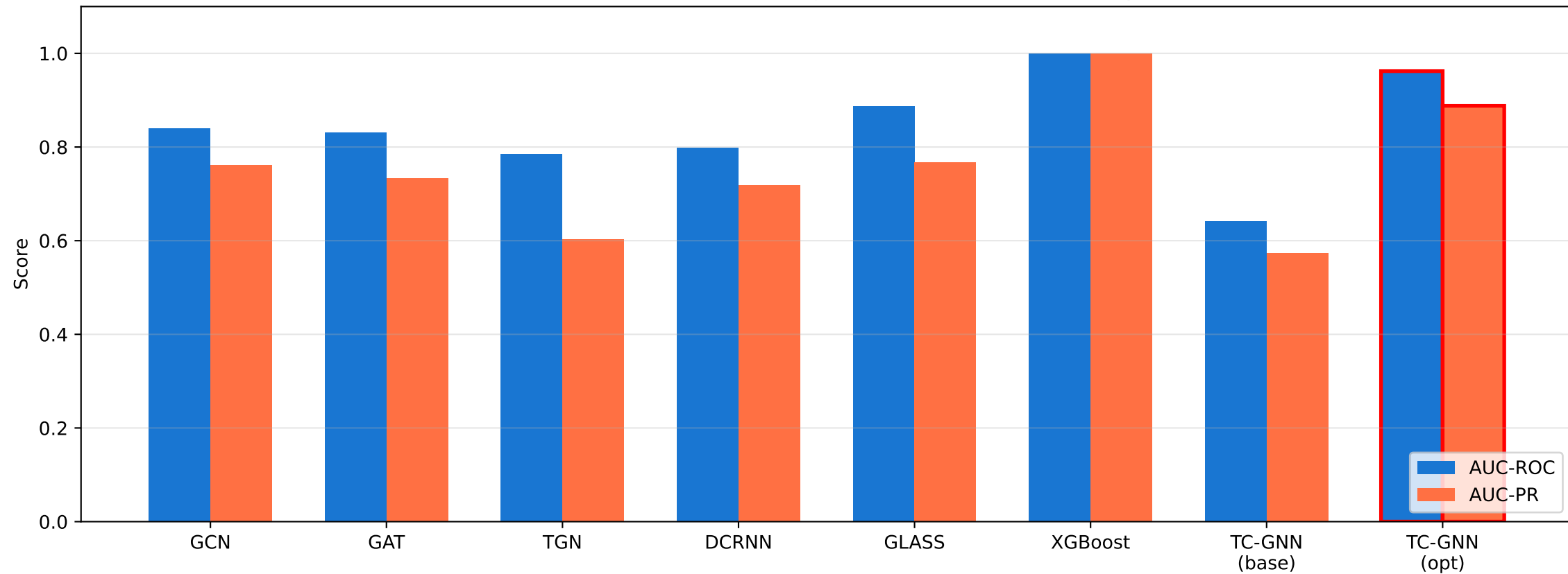
Headline cycle-level detection on REAL Elliptic1 (165-dim features, near-miss negatives, 1K candidates, 30 epochs)
