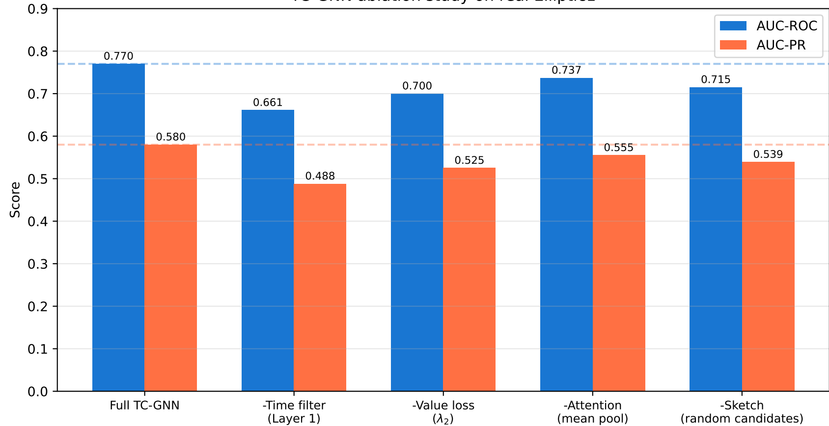
TC-GNN ablation study on real Elliptic1
