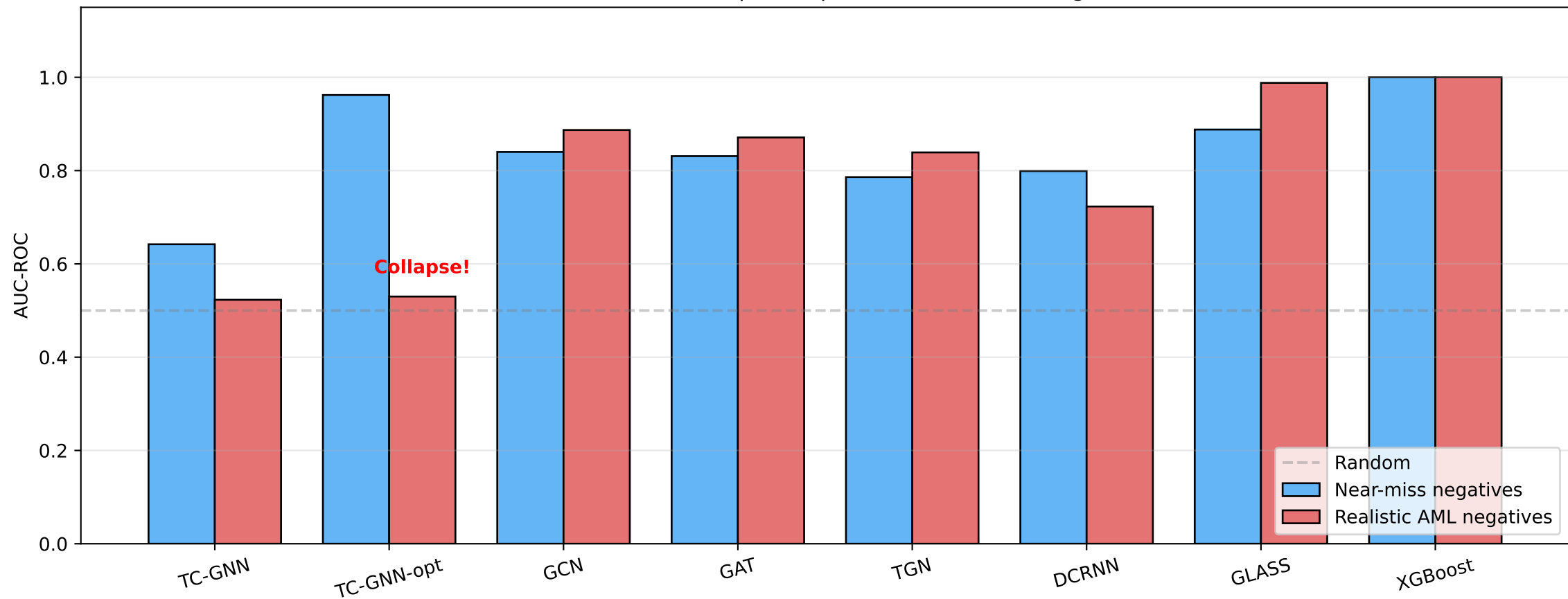
Stress test: TC-GNN-opt collapses under realistic negatives
