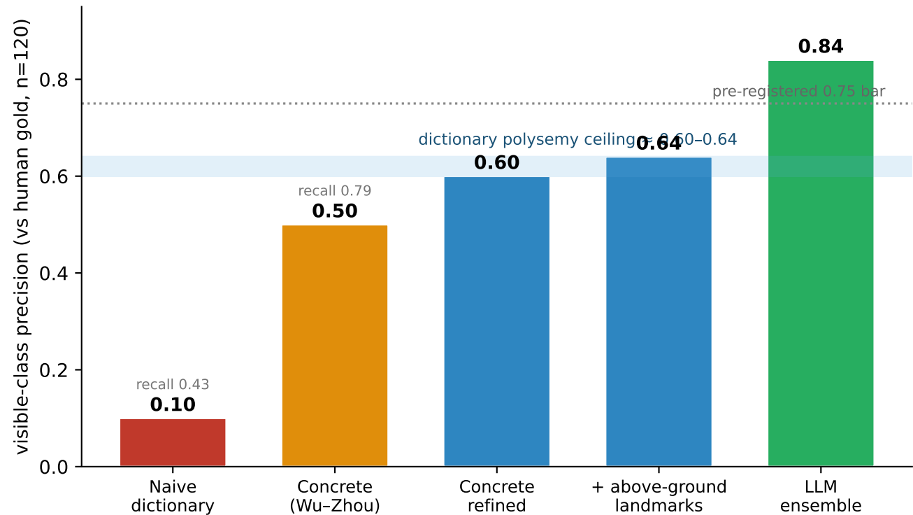
Lexicon precision ladder: curation hits a polysemy ceiling; LLM ensemble clears it
