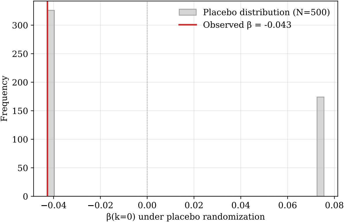
Placebo test: observed effect vs randomized-treatment null (two-tailed p = 1.000)
