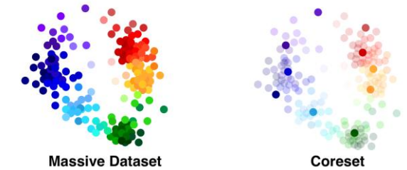
Coreset Selection
