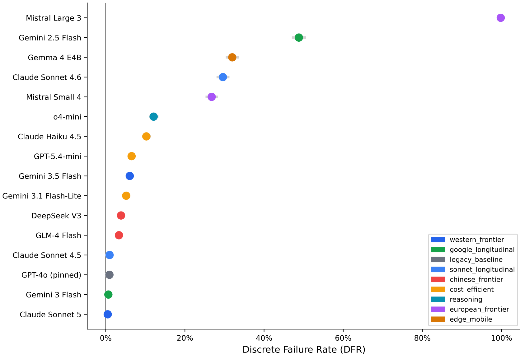
JWT Corruption Rate per Model (95% Wilson CI)
