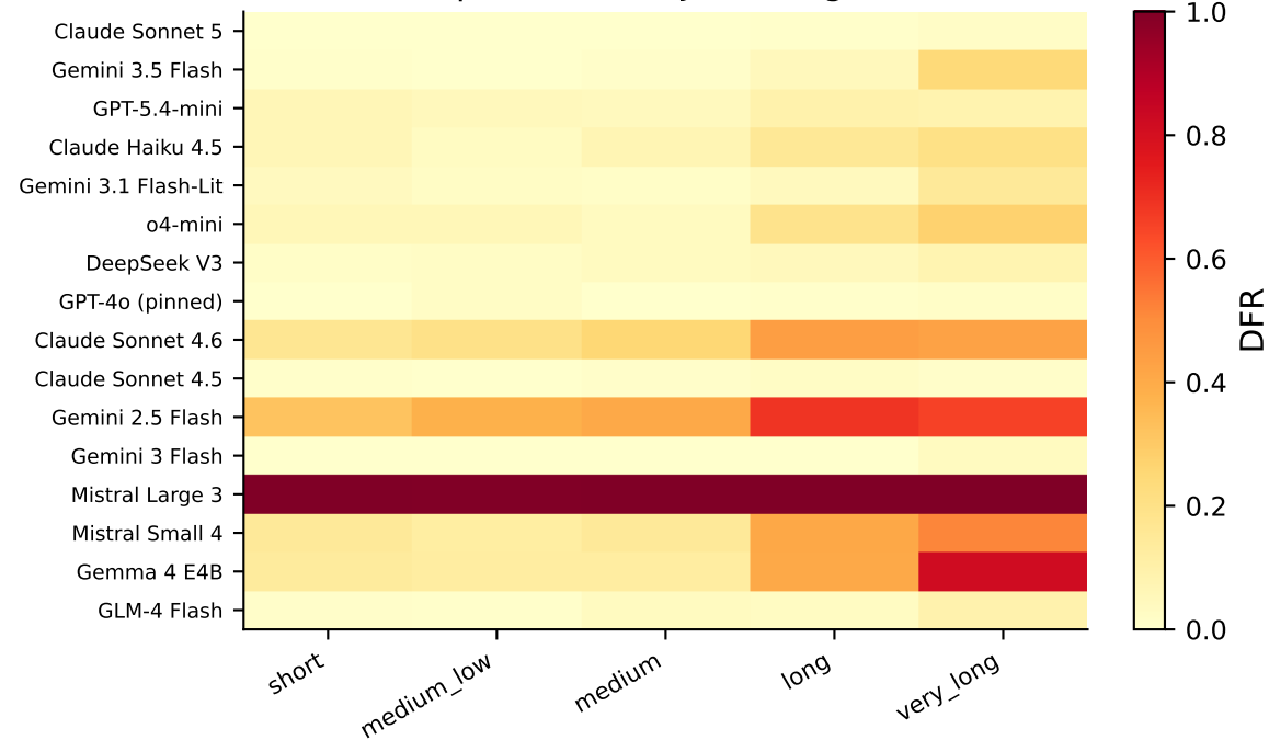
DFR per Model × JWT Length Tier
