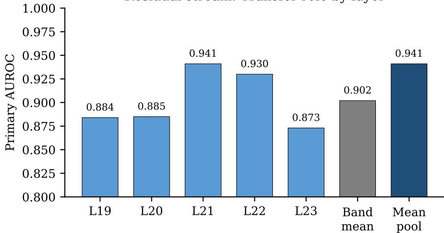
Residual stream: Transfer role by layer
