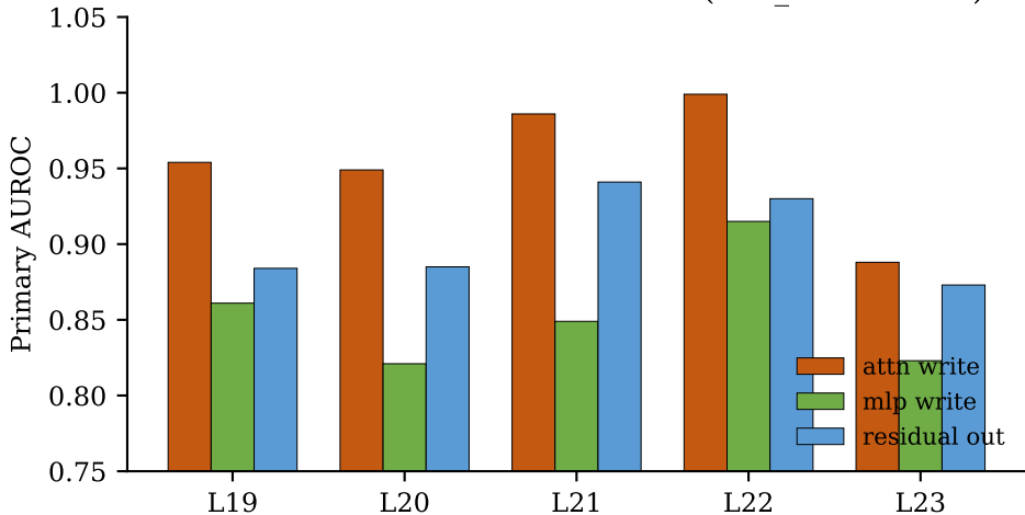
Block write-in: attention dominates ( \text{attn\_L22} \approx 0.999 )
