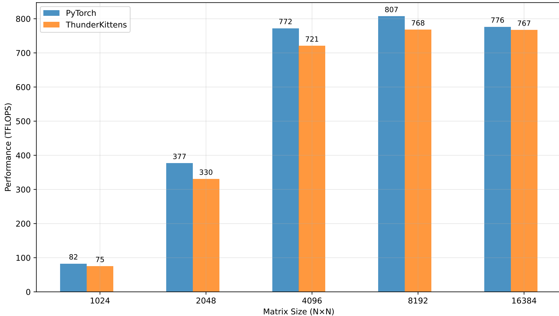
BF16 GEMM Performance Comparison MI325X
