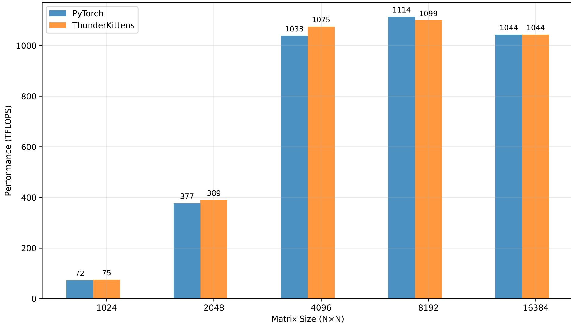
BF16 GEMM Performance Comparison MI350X
