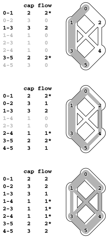
Figure 22.6 Controlling flow in a network
