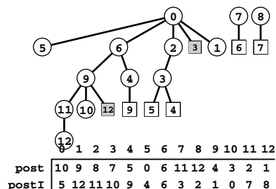
Figure 19.24 DFS forest for a DAG
