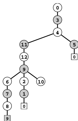
Figure 18.15 Two-coloring a DFS tree
