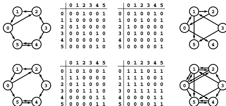
Figure 19.14 Squaring an adjacency matrix
