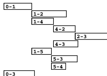
Figure 21.25 A PERT chart
