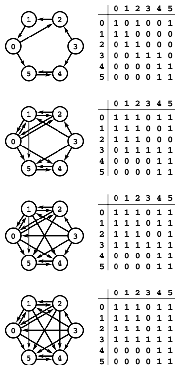
Figure 19.15 Adjacency matrix powers and directed paths
