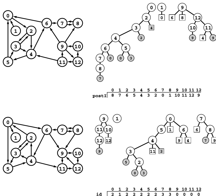
Figure 19.28 Computing strong components (Kosaraju's algorithm)
