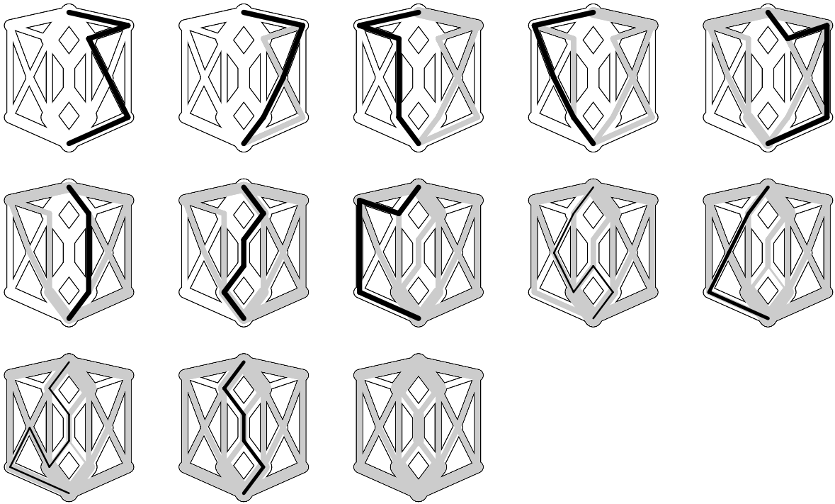
Figure 22.20 Stack-based augmenting-path search
