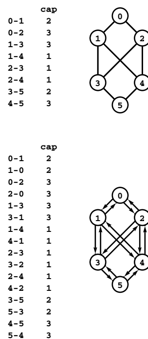
Figure 22.34 Reduction from undirected networks
