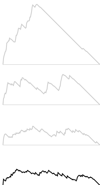
Figure 20.11 Fringe size for PFS implementation of Prim's algorithm
