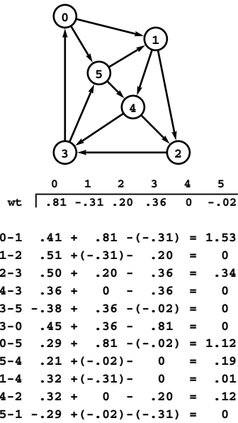
Figure 21.31 Reweighting a network
