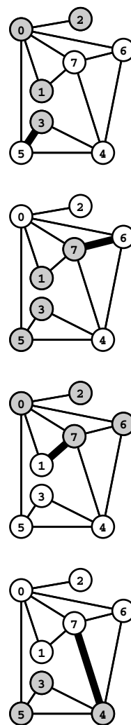
Figure 20.5 Cut property
