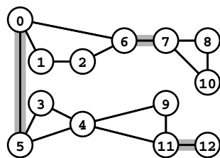
Figure 18.16 An edge-separable graph
