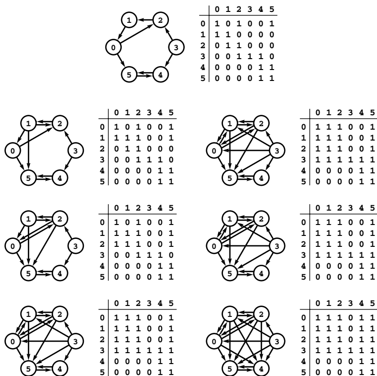
Figure 19.16 Warshall's algorithm
