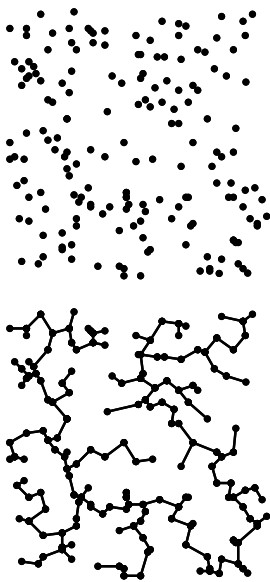
Figure 20.18 Euclidean MST
