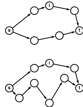
Figure 21.7 Path relaxation
