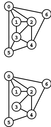
Figure 17.18 Hamilton tour
