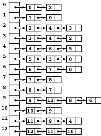
Figure 19.5 Digraph reversal
