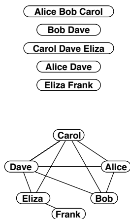
Figure 17.15 Degrees-of-separation graph
