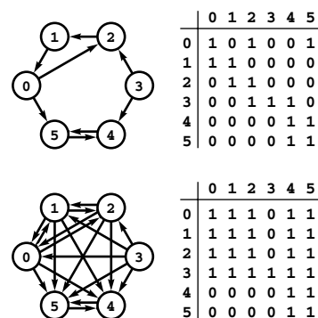
Figure 19.13 Transitive closure
