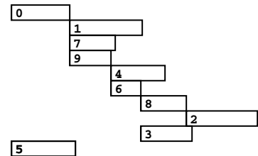
Figure 21.24 Job schedule
