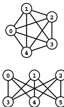
Figure 17.24 Forbidden subgraphs in planar graphs
