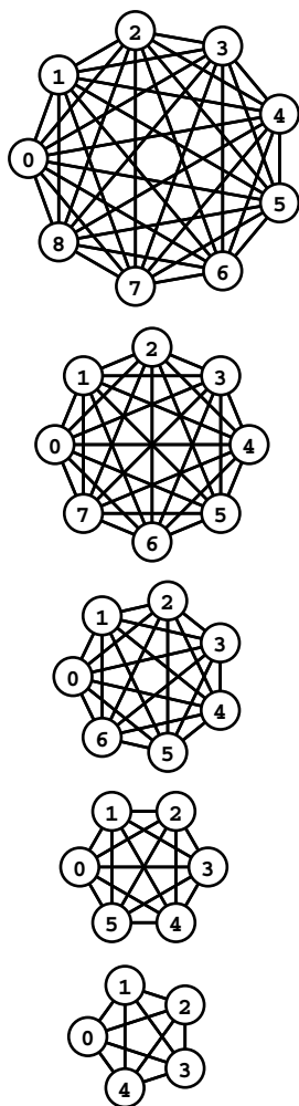
Figure 17.4 Complete graphs
