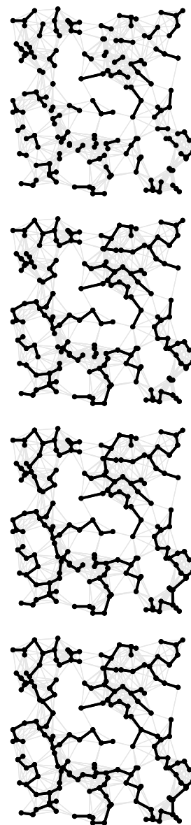
Figure 20.16 Boruvka's MST algorithm
