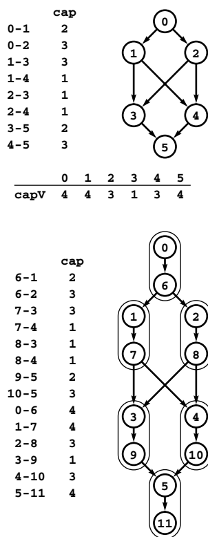
Figure 22.32 Removing vertex capacities
