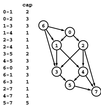
Figure 22.36 Reduction from feasible flow
