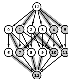
Figure 22.33 Reduction to acyclic network
