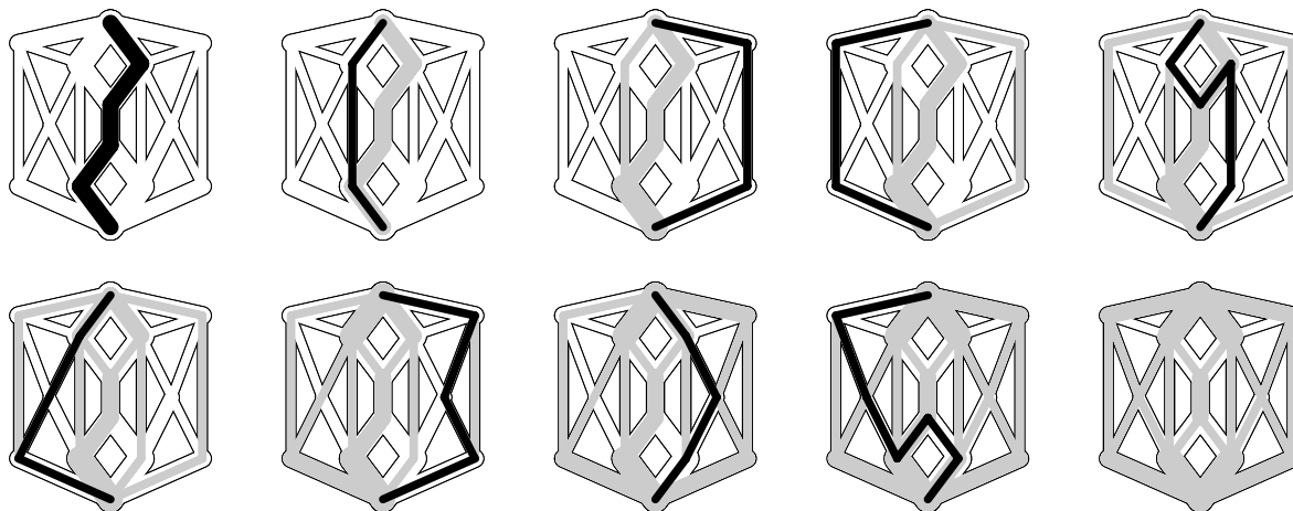
Figure 22.18 Maximum-capacity augmenting paths
