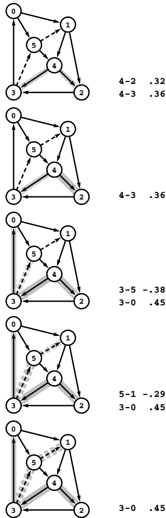
Figure 21.28 Failure of Dijkstra's algorithm (negative weights)
