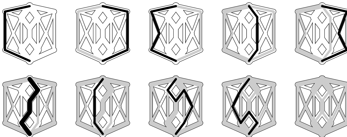
Figure 22.21 Randomized augmenting-path search
