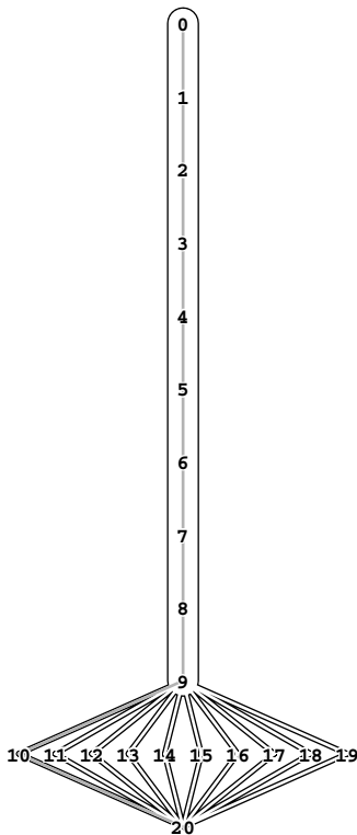
Figure 22.26 Bad case for the Ford–Fulkerson algorithm
