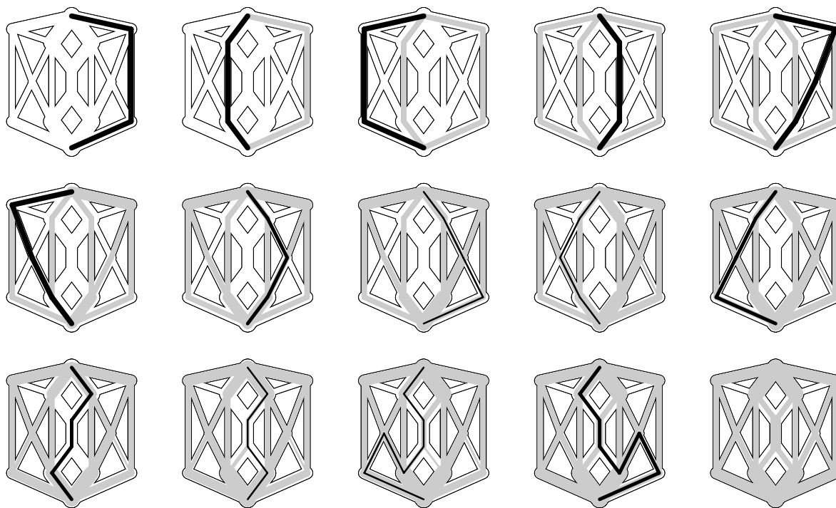
Figure 22.17 Shortest augmenting paths
