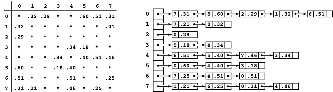
Figure 20.3 Weighted-graph representations (undirected)
