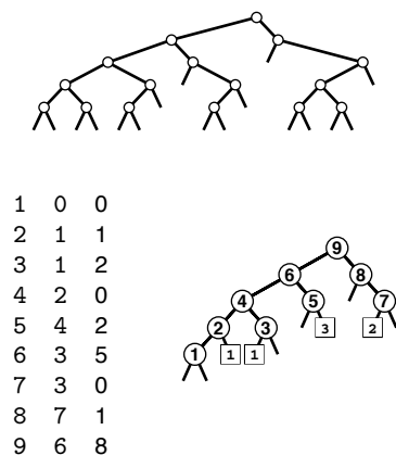
Figure 19.20 Binary tree compression
