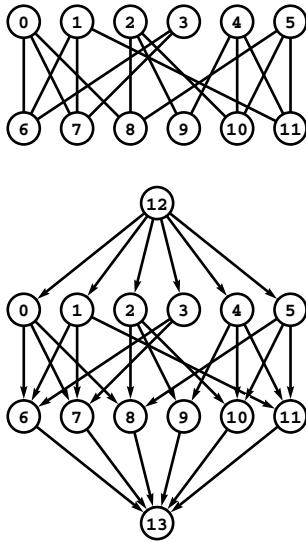
Figure 22.38 Reduction from bipartite matching
