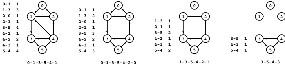
Figure 22.9 Cycle flow decomposition process
