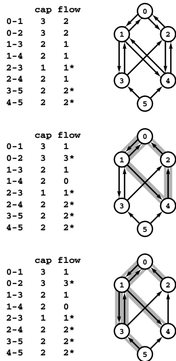
Figure 22.44 Maxflow spanning tree
