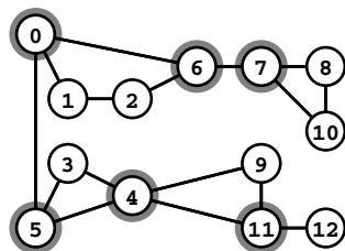
Figure 18.20 Articulation points (separation vertices)
