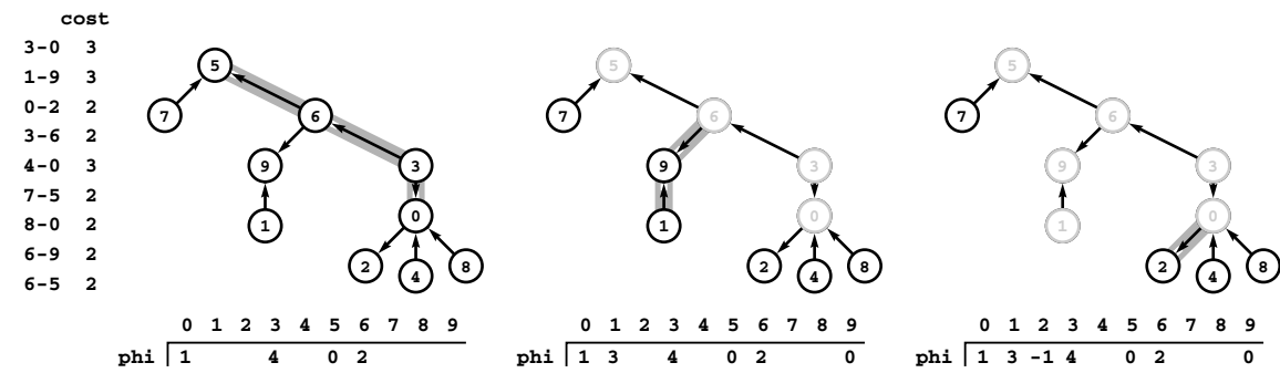
Figure 22.47 Computing potentials through parent links
