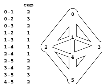
Figure 22.10 Flow network for exercises
