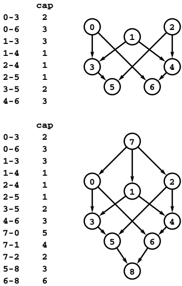
Figure 22.31 Reduction from multiple sources and sinks
