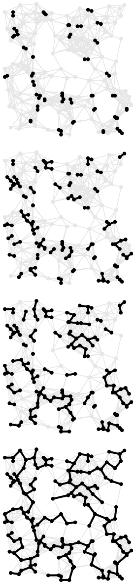
Figure 20.13 Kruskal's MST algorithm
