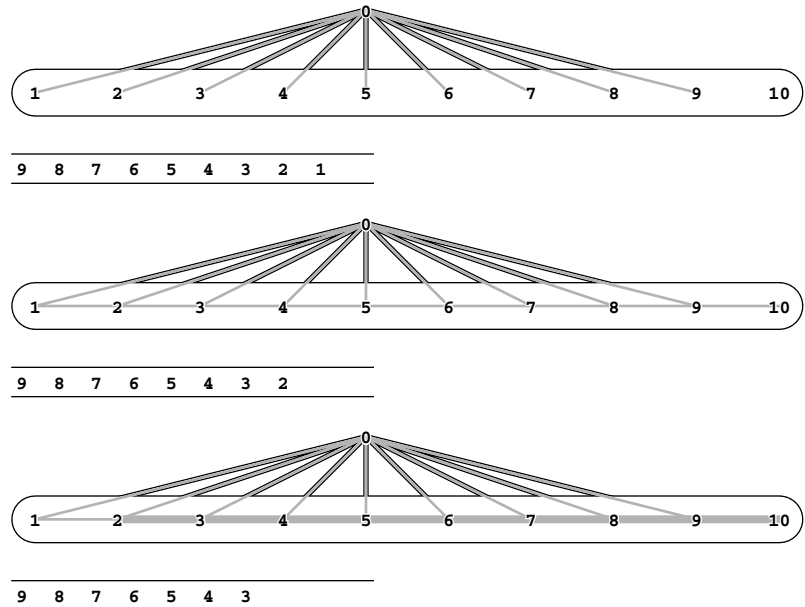
Figure 22.29 FIFO preflow-push worst case
