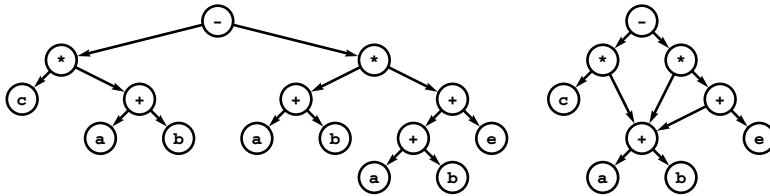
Figure 19.19 DAG representation of an arithmetic expression
