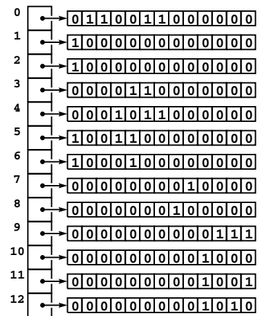
Figure 17.9 Adjacency matrix data structure
