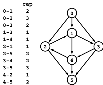
Figure 22.11 Flow network with cycle
