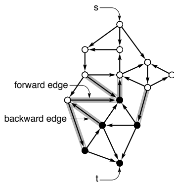
Figure 22.14 st -cut terminology
