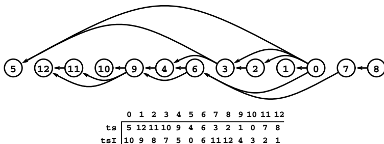
Figure 19.23 Reverse topological sort
