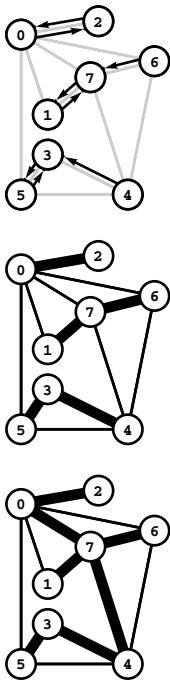
Figure 20.14 Boruvka's MST algorithm
