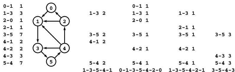
Figure 22.8 Cycle flow representation
