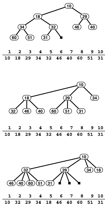
Figure 20.17 2-, 3-, and 4-ary heaps
