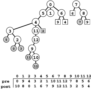
Figure 19.9 DFS forest for a digraph
