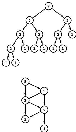
Figure 19.18 DAG model of Fibonacci computation
