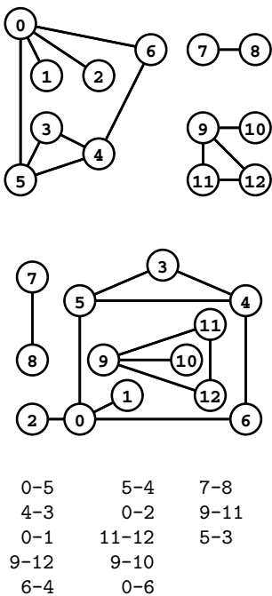
Figure 17.1 Three different representations of the same graph
