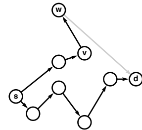
Figure 21.18 Edge relaxation (Euclidean)
