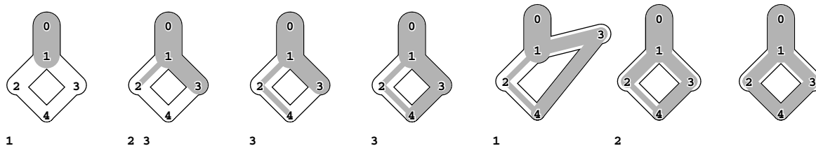
Figure 22.25 Preflow-push example
