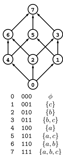
Figure 19.17 Set-inclusion DAG
