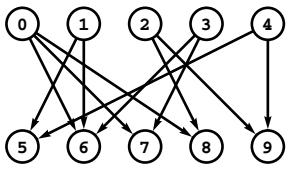
Figure 22.2 Transportation problem
