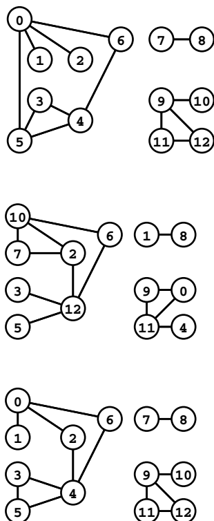
Figure 17.2 Graph isomorphism examples
