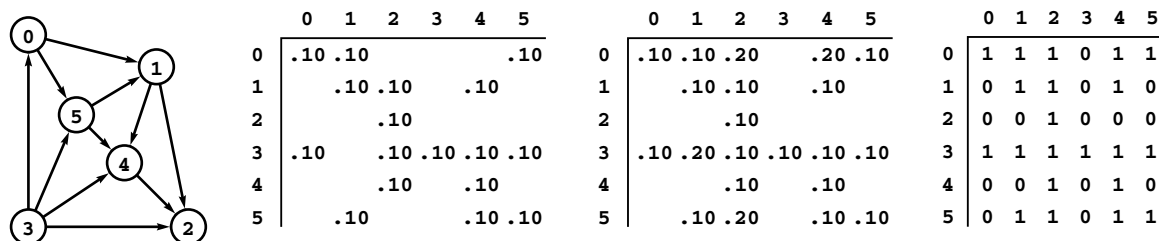
Figure 21.21 Transitive-closure reduction
