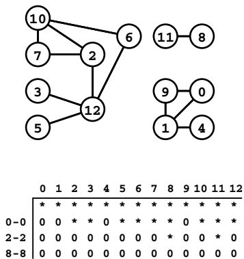
Figure 18.8 Graph search
