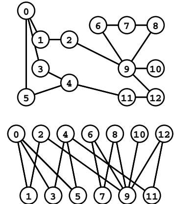
Figure 17.5 A bipartite graph
