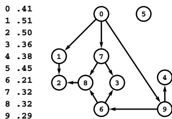
Figure 21.22 Job scheduling
