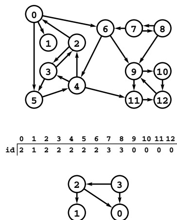
Figure 19.8 Strong components and kernel DAG
