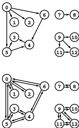
Figure 17.6 Two digraphs
