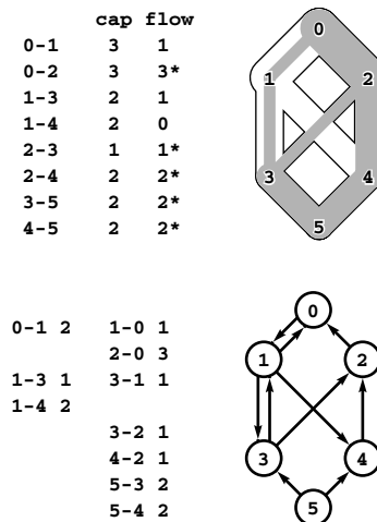
Figure 22.43 Edge classification
