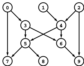
Figure 22.1 Distribution problem
