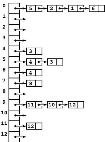
Figure 17.11 Digraph representations
