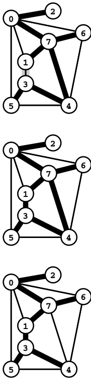
Figure 20.6 Cycle property
