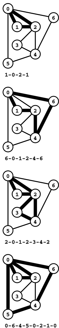
Figure 17.22 Partial tours
