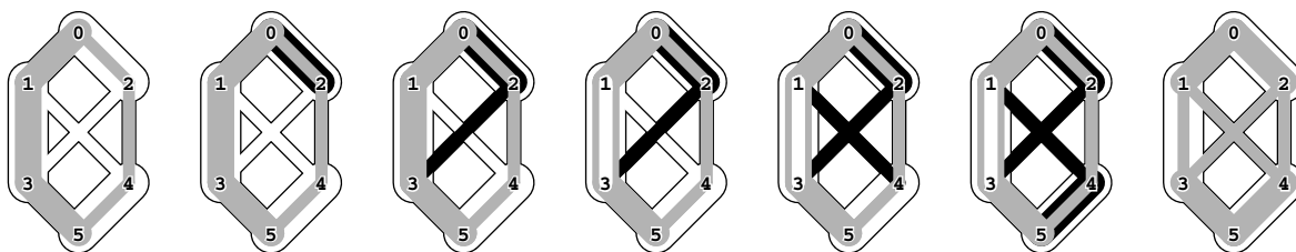
Figure 22.12 Augmenting flow along a path
