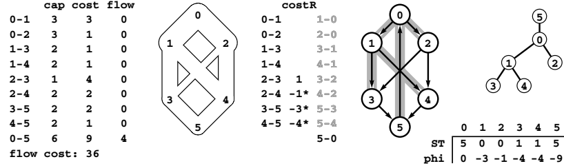
Figure 22.49 Network simplex initialization
