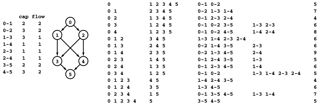
Figure 22.15 All st -cuts
