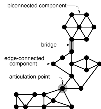
Figure 18.19 Graph separability terminology
