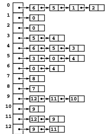
Figure 17.10 Adjacency-lists data structure
