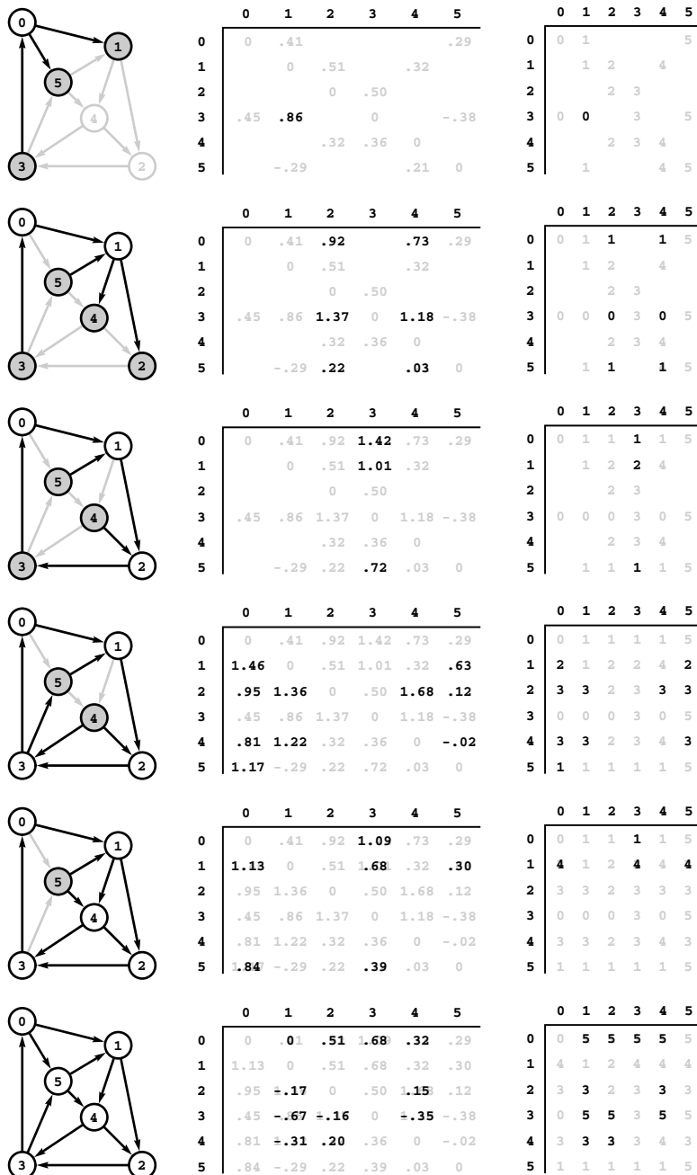
Figure 21.29 Floyd's algorithm (negative weights)
