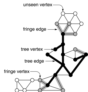
Figure 18.26 Graph search terminology
