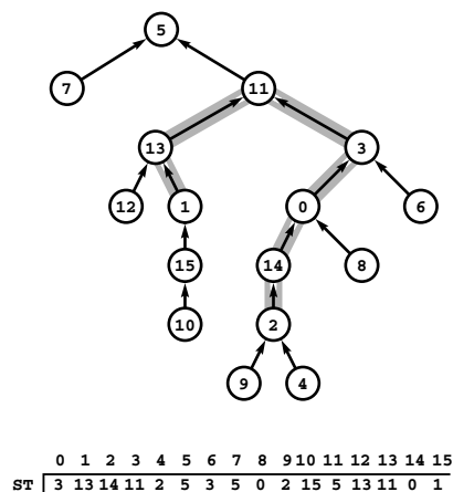
Figure 22.48 Spanning tree substitution
