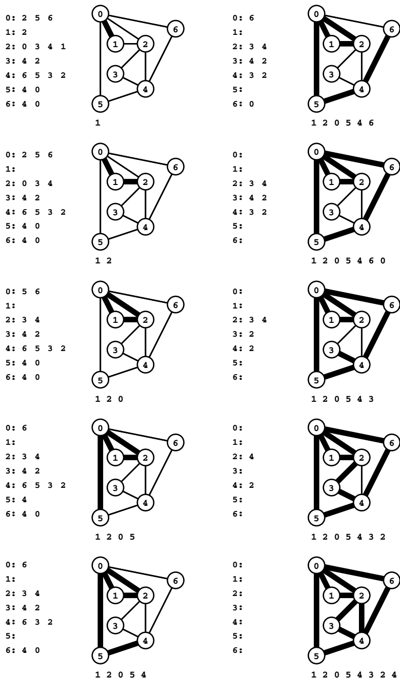
Figure 17.23 Euler tour by removing cycles
