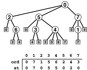
Figure 18.22 BFS tree
