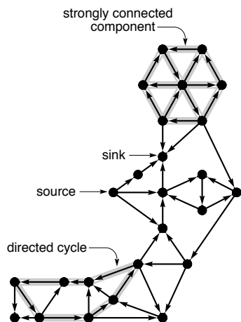
Figure 19.7 Digraph terminology
