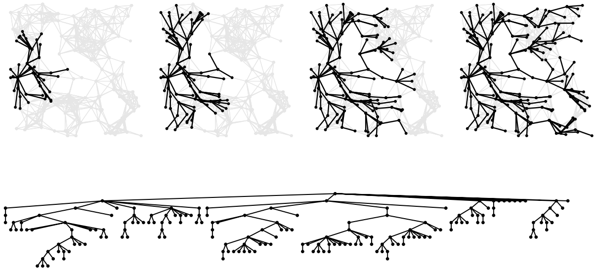
Figure 18.24 Breadth-first search
