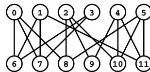
Figure 22.37 Bipartite matching
