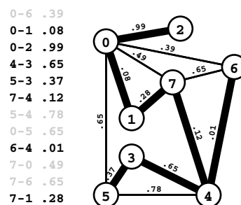
Figure 20.2 Arbitrary weights
