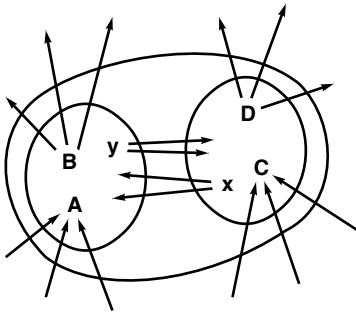
Figure 22.7 Flow equilibrium
