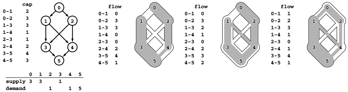
Figure 22.35 Feasible flow
