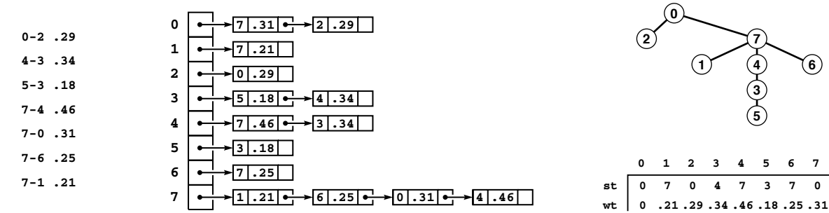
Figure 20.4 MST representations
