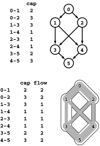
Figure 22.5 Network flow
