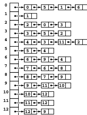
Figure 19.4 Digraph representations
