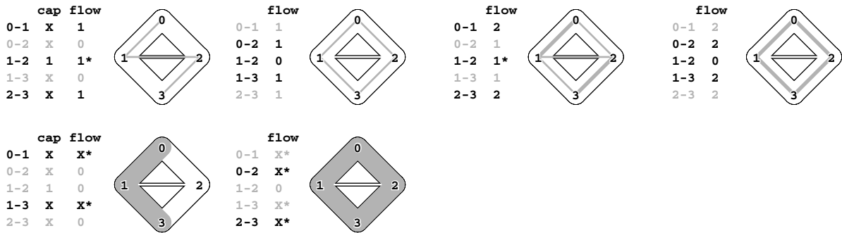
Figure 22.19 Two scenarios for the Ford-Fulkerson algorithm
