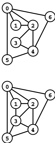
Figure 17.20 Euler tour and path examples
