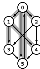
Figure 22.45 Spanning tree for dummy maxflow
