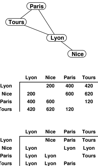
Figure 21.4 Distances and paths
