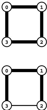
Figure 20.7 Cycles in Boruvka's algorithm
