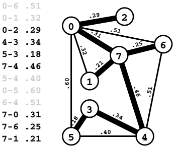
Figure 20.1 A weighted undirected graph and its MST
