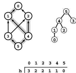
Figure 22.27 Initial height function
