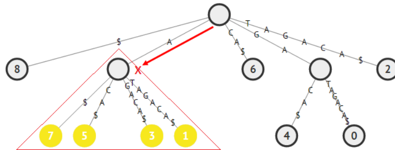
Figure 6.4: String Matching of T = \text{"GATAGACA\$"}^{\text{14}} with Pattern String P = \text{"A"}^{\text{15}}
