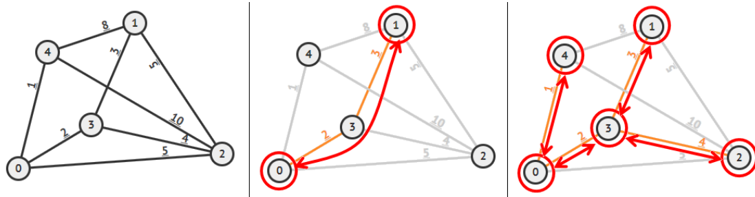
Figure 8.34: Steiner Tree Illustrations—Part 1
