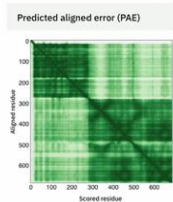
Model Confidence
