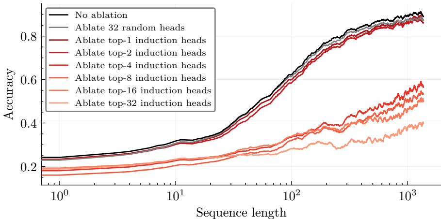
Ablating induction heads
