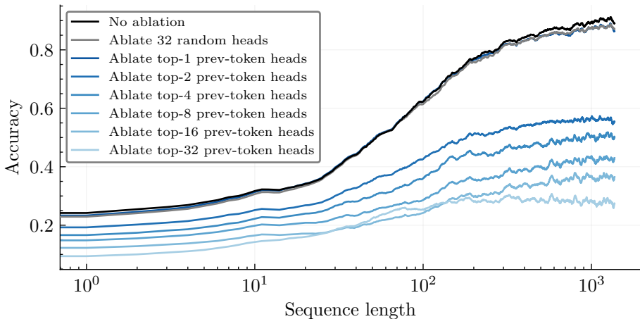
Ablating previous-token heads
