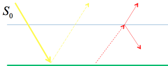
Figure 1.1: A schematic of the Energy Balance Model (EBM), a conceptual climate model based on the conservation of energy. S_0 , represented by the yellow arrow, represents energy coming from the sun absorbed by Earth’s surface (horizontal green bar). The red, dashed arrow represents energy radiating out of Earth’s surface, of which some is reflected back by the atmosphere (horizontal gray line). Since energy is conserved in the EBM, the parameterizations of surface albedo (amount reflected by Earth’s surface), atmospheric absorptivity, and radiation rate determine the long term behavior of internal energy (temperature). This schematic was provided in a lecture given by Dr. Chris Jones (?).
