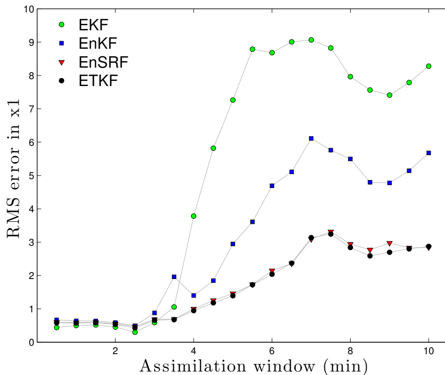
Figure 2.9: The RMS error (not scaled by climatology) is reported for our EKF and EnKF filters, measured as the difference between forecast and truth at the end of an assimilation window for the latter 2500 assimilation windows in a 3000 assimilation window model run. Error is measured in the only observed variable, x_1 . Increasing the assimilation window led to a decrease in predictive skill, as expected. Additive and multiplicative covariance inflation is the same as Harris et al. (2011).
