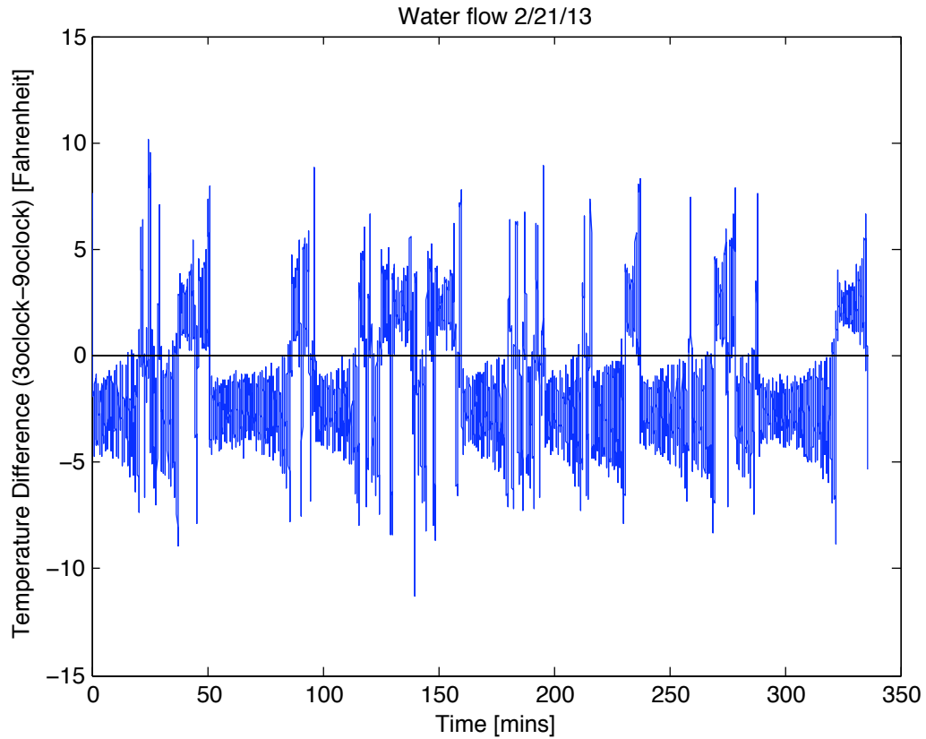
Figure 4.3: A time series of the physical thermosyphon, from the Undergraduate Honor's Thesis of Darcy Glenn (Glenn 2013). The temperature difference (plotted) is taken as the difference between temperature sensors in the 3 and 9 o'clock positions. The sign of the temperature difference indicates the flow direction, where positive values are clockwise flow.
