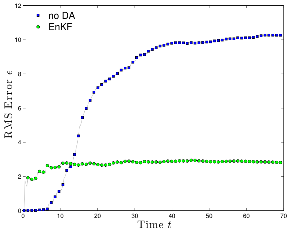
Figure 2.6: For near-perfect initial knowledge of the atmospheric state, the running average RMS error of a prediction using DA is compared against a prediction that does not. Initial error for DA is normal with mean 0 and variance 0.01, and the RMS errors reported are averages of 100 runs. Observational noise is normally distributed with mean 0 and variance 0.5 (approximately 5% of climatological variation), and an assimilation window length of 0.261 is used. As would be expected, in the long run DA greatly improves forecast skill, as forecasts without DA saturate to climatological error. The initial period where a forecast exceeds the skill of DA is potentially due to the spin-up time required by the filter to dial in the analysis error covariance.
