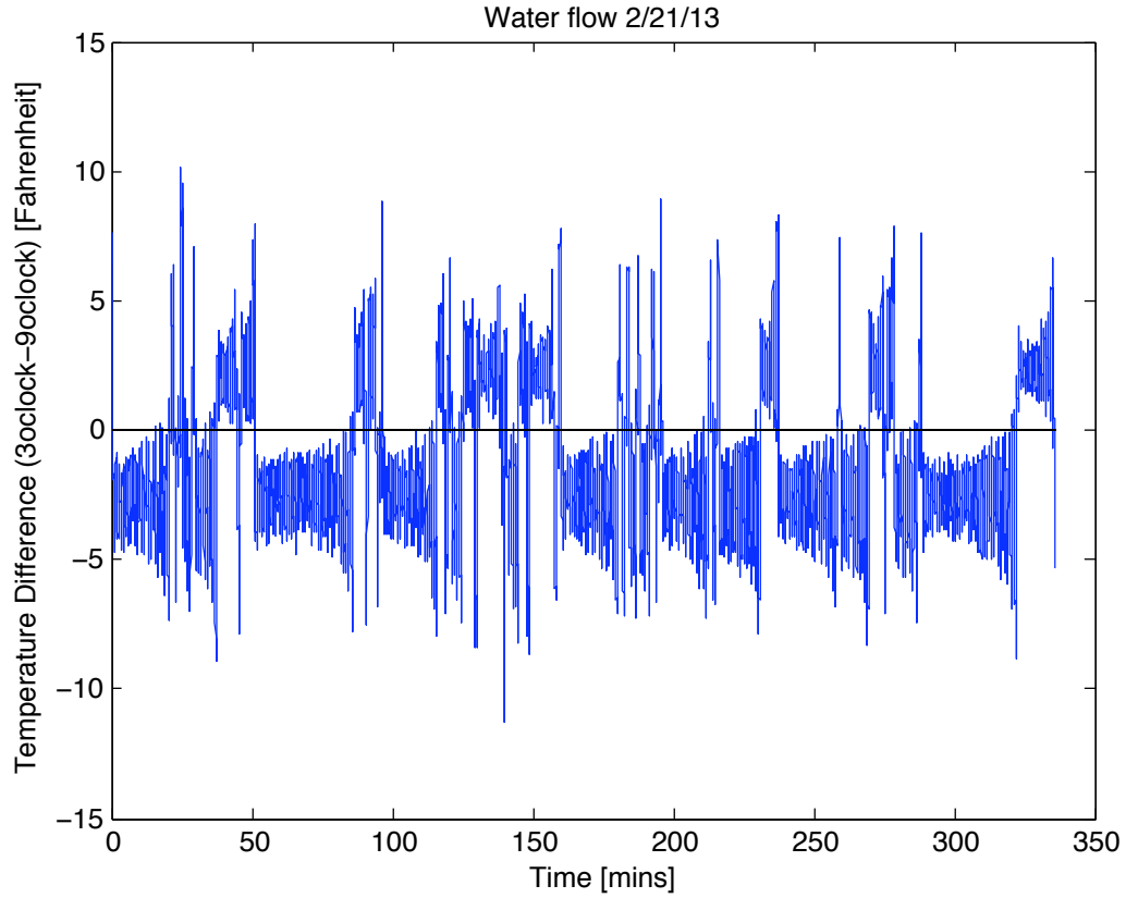
Figure 3.4: A time series of the physical thermosyphon, from the Undergraduate Honor's Thesis of Darcy Glenn (Glenn 2013). The temperature difference (plotted) is taken as the difference between temperature sensors in the 3 and 9 o'clock positions. The sign of the temperature difference indicates the flow direction, where positive values are clockwise flow.
