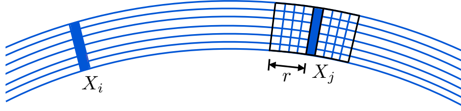
Figure 4.3: covariance localization zones
