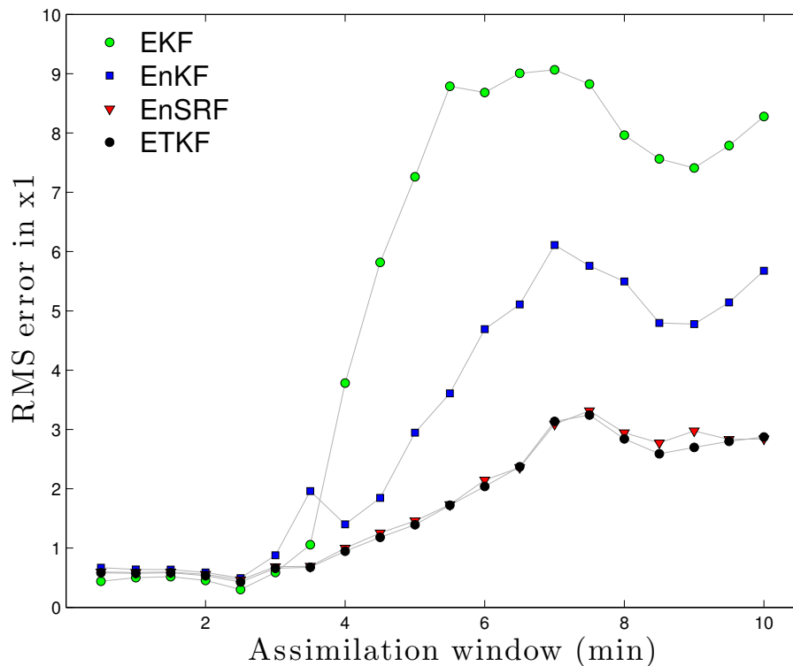
Figure 4.1: A first pass (covariance inflation not tuned) experiment of Lorenz 63 (EM) prediction skill vs increasing assimilation windows on real data. Notice that the error explodes at an window length near the typical time length of flow reversals.
