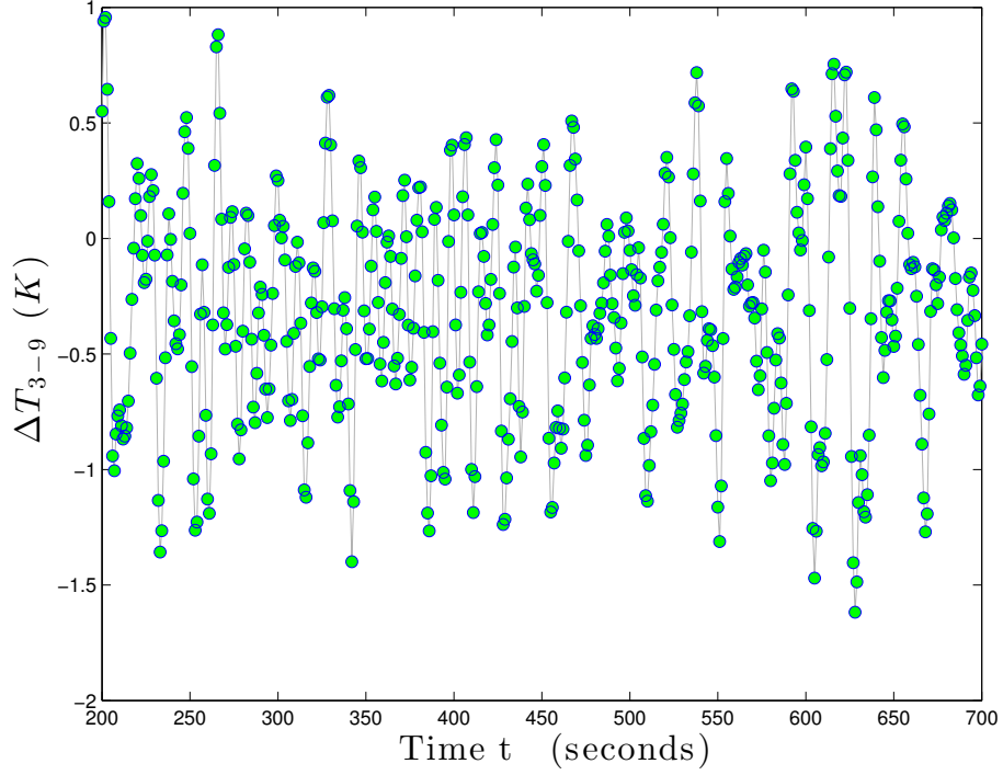
Figure 4.2: The CFD generated timeseries used as synthetic data to test predictions.
