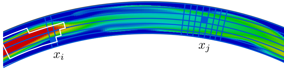
Figure 4.8: covariance localization adaptive
