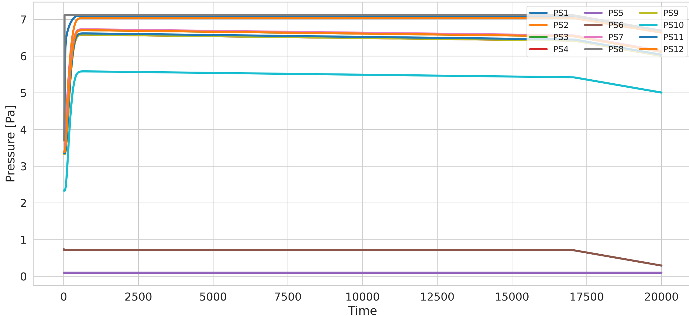
Pressure Sensors - Normality Scenario (Gest Down)
