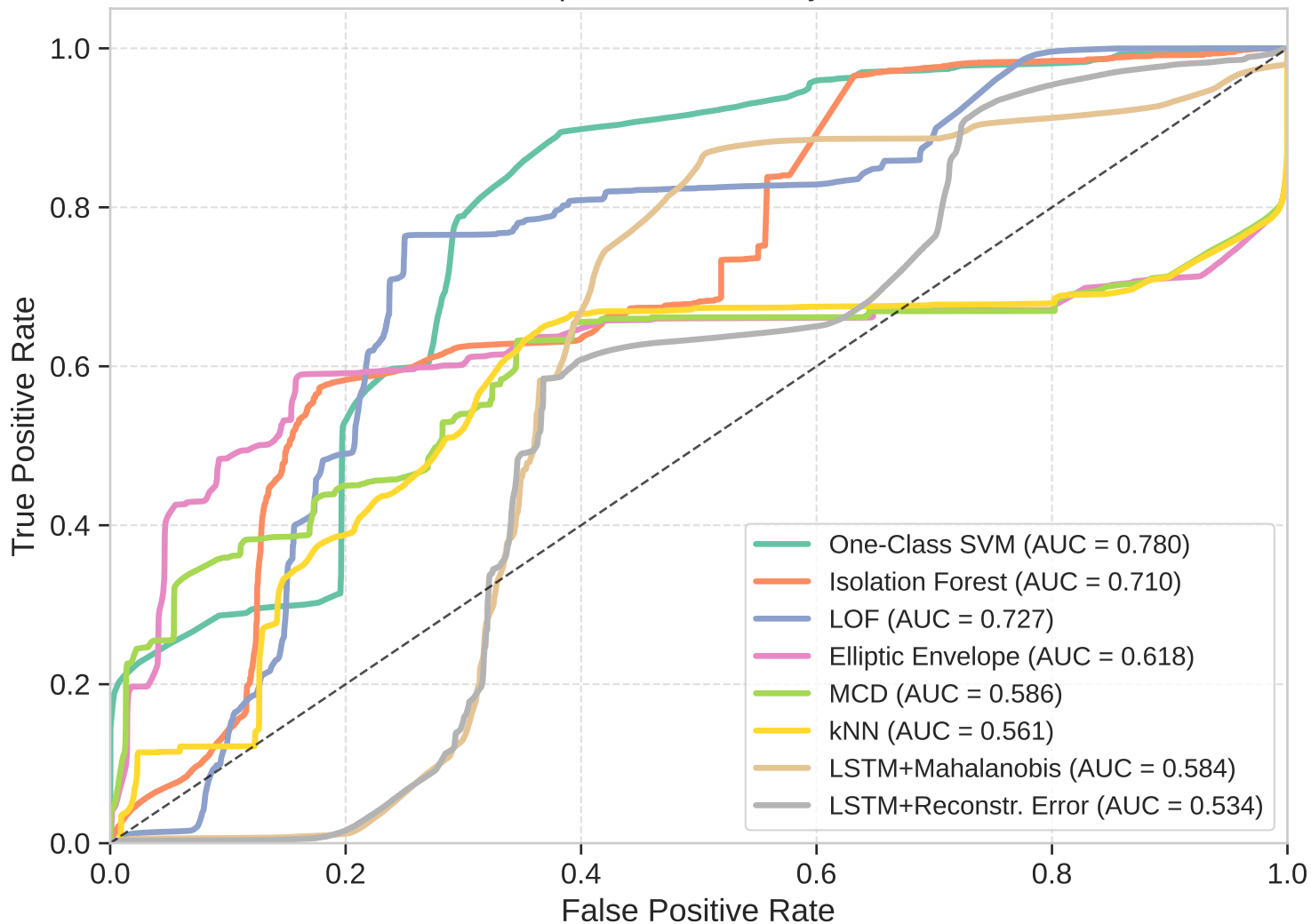
ROC Curve Comparison - Anomaly Detection Models
