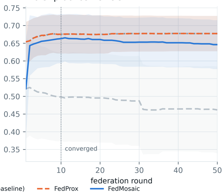
Worst-practice AUROC
