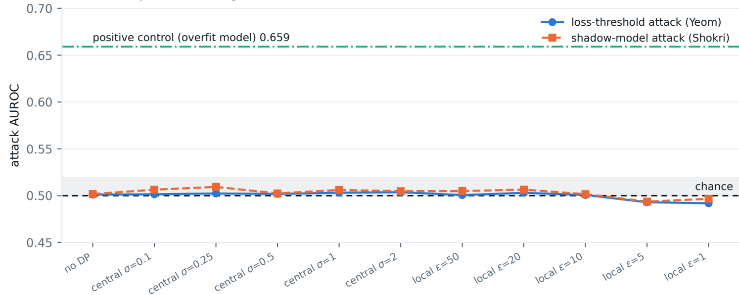
Membership inference against the released model
