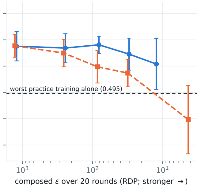
Worst-practice AUROC
