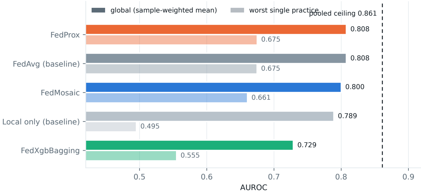
Global vs worst-practice AUROC · 20 rounds, 5 seeds
