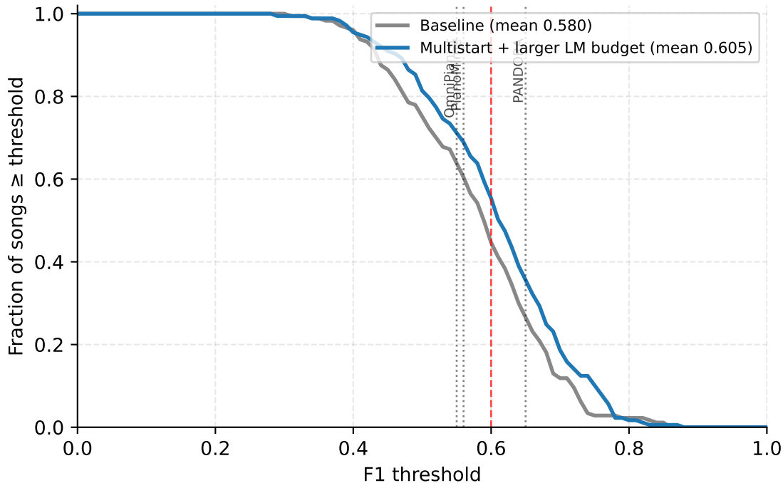
Cumulative F1 distribution on MAESTRO v3 test split (177 songs)
