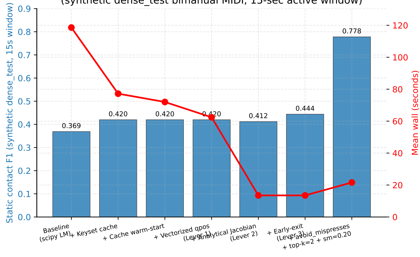
Architectural ablation: cumulative F1 lift and wall reduction (synthetic dense_test bimanual MIDI, 15-sec window)
