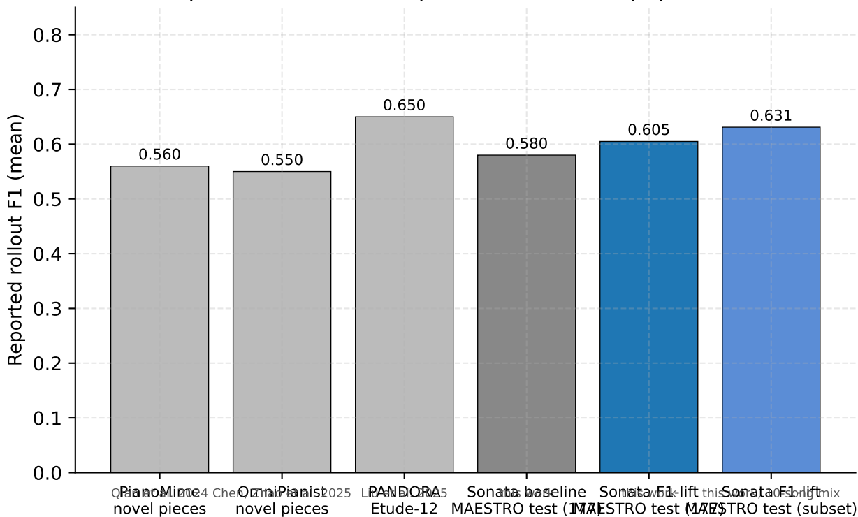
Reported F1 across methods (NOT apples-to-apples in eval conditions) Baselines reported on different splits/datasets; see paper text for caveats
