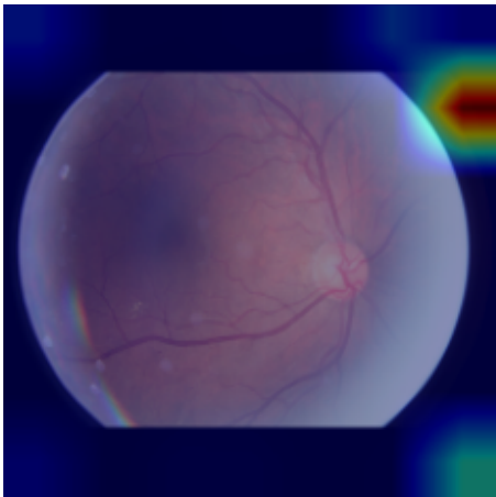
EfficientNet-B4 Grad-CAM Pred: Moderate (0.44) Wrong
