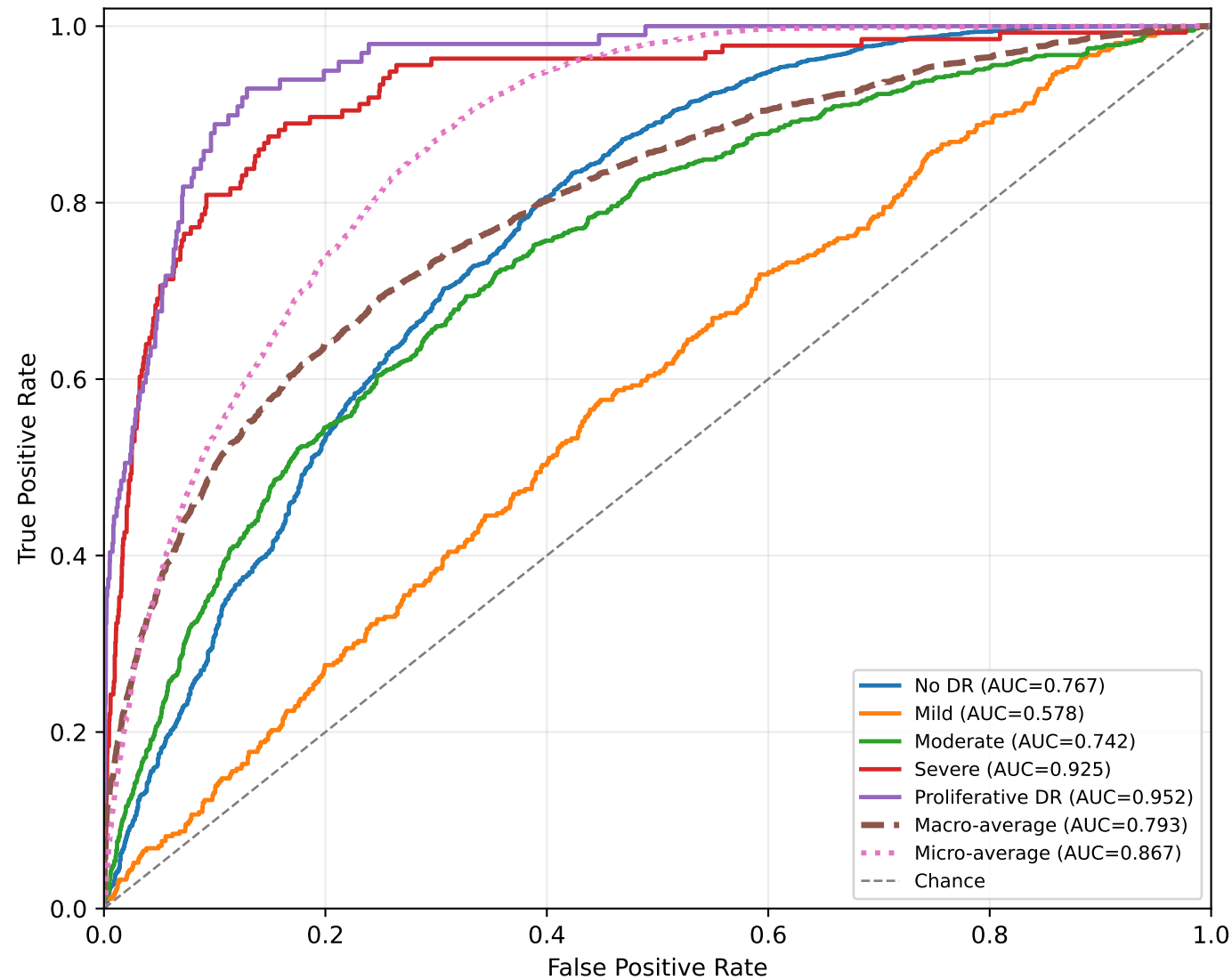
EfficientNet-B4: one-vs-rest ROC curves
