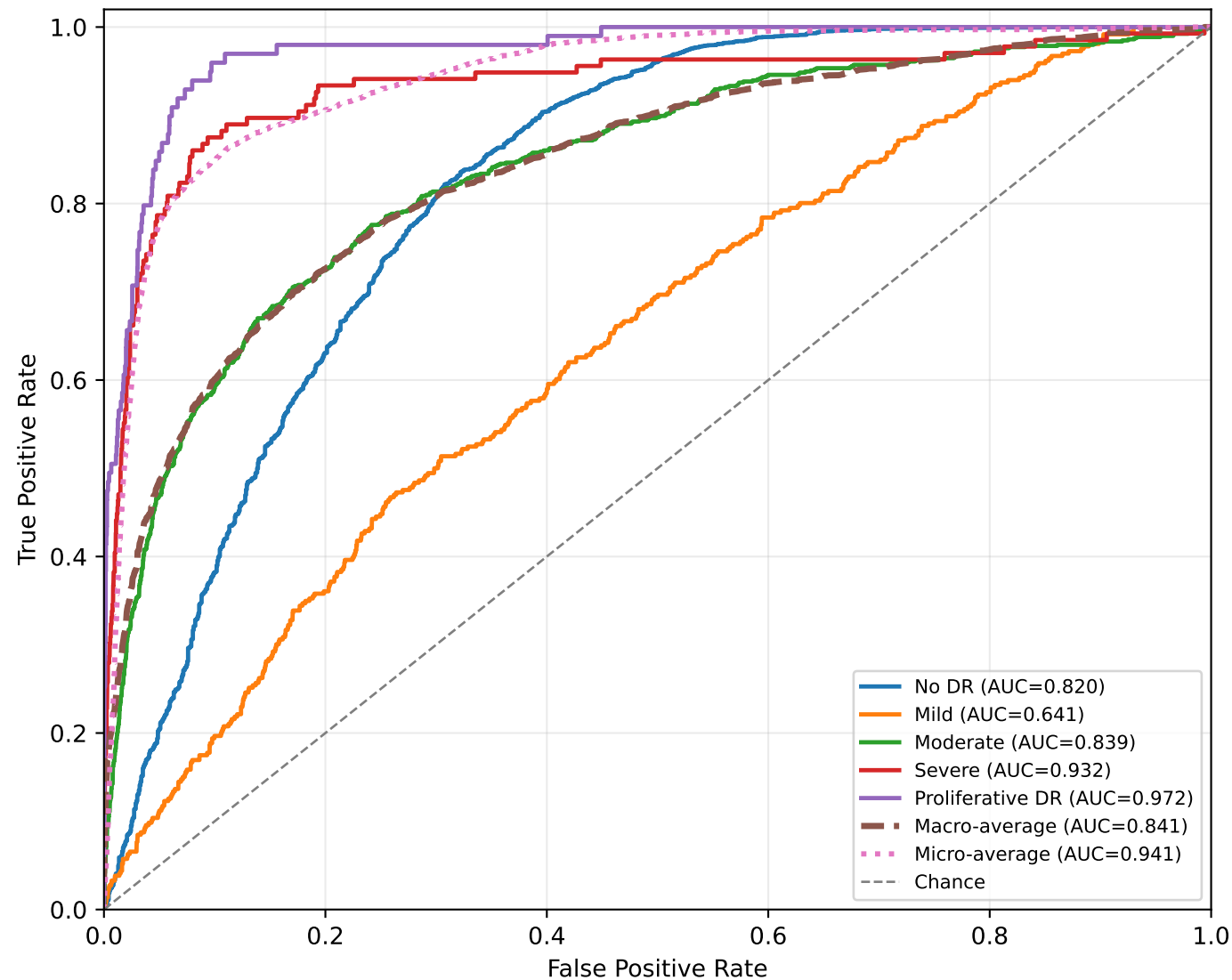
DeiT-III-B/16: one-vs-rest ROC curves
