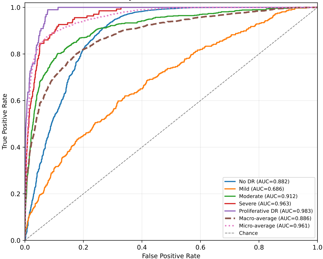
MaxViT-Tiny M12: one-vs-rest ROC curves
