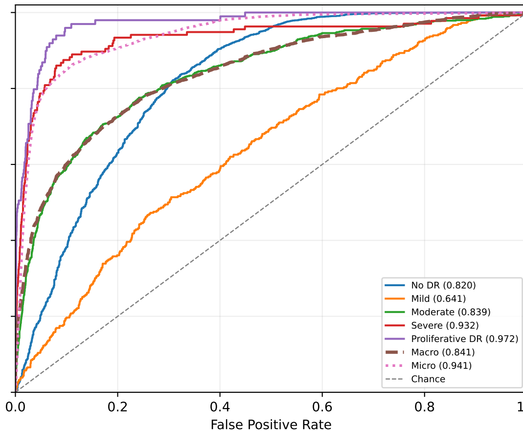
(b) DeiT-III-B/16
