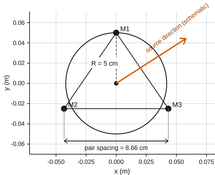
Figure 1. Microphone geometry and matched simulation controls. (a) Layout of the equilateral three-microphone array with circumradius R = 5\text{ cm} and inter-microphone spacing of 8.66\text{ cm} . The microphone coordinates are drawn to scale; the arrow shows one tested source azimuth and is not drawn to the 1.5\text{ m} source distance. (b) The three matched binary controls form eight combinations. Within each scene and recording, every combination uses identical source and microphone-noise samples. Onset denotes one source startup at the beginning of the complete recording.
