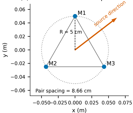
(a) Horizontal three-microphone array
