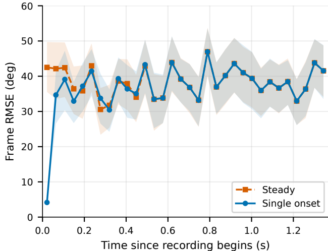
(b) High subset: source-history effect
